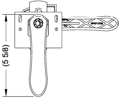
7 TUFF SHED "L" HANDLE VENDOR: SIERRA PACIFIC PART #390209 SCALE: 3" = 1'-0"
