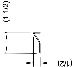
16 STRIKE PLATE VENDOR: SIERRA PACIFIC SCALE: 3" = 1'-0"
