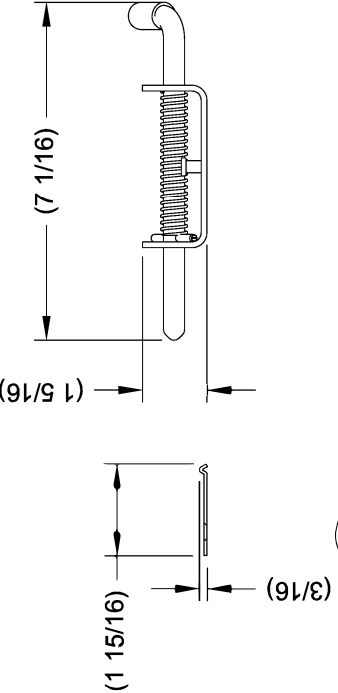
17 HURRICANE SPRING BOLT VENDOR: SIERRA PACIFIC PART #1147ZN SCALE: 3" = 1'-0"
